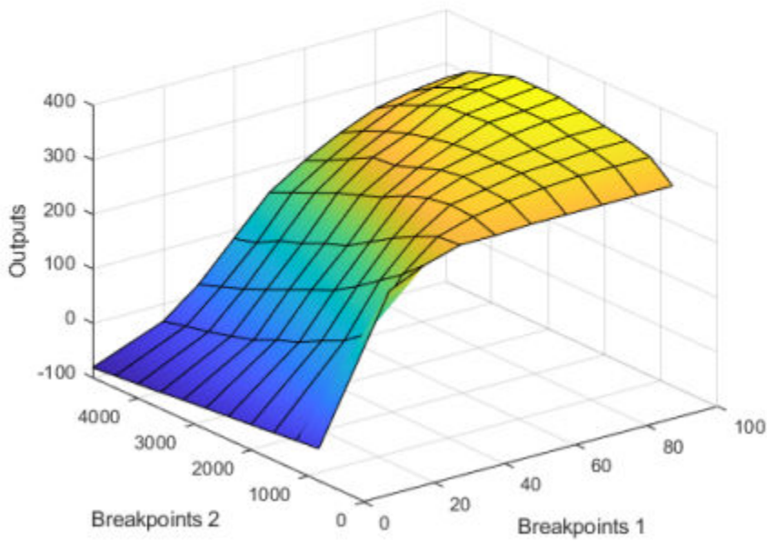
Figure 5.1. engine torque (:,:)
